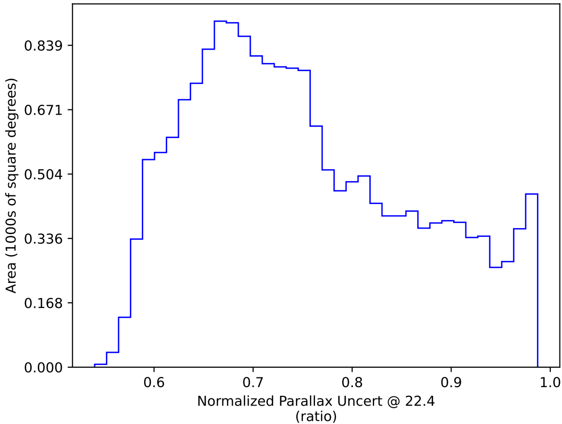
too_5_4v3.4_10yrs WFD: Normalized Parallax Uncert @ 22.4
