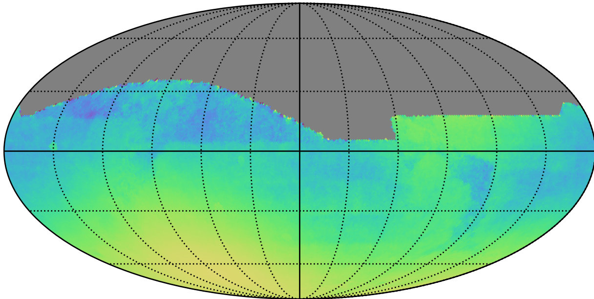
too_5_4v3.4_10yrs All sky: Normalized Parallax Uncert @ 22.4
