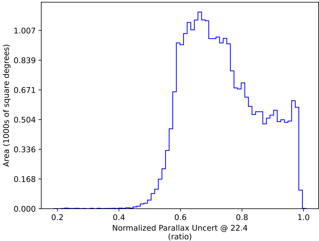
too_5_4v3.4_10yrs All sky: Normalized Parallax Uncert @ 22.4
