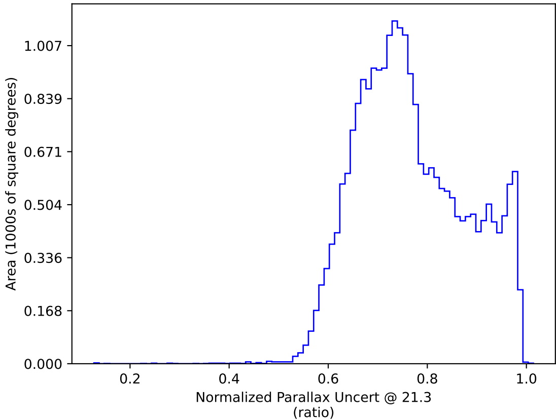
too_5_4v3.4_10yrs All sky y band only: Normalized Parallax Uncert @ 21.3
