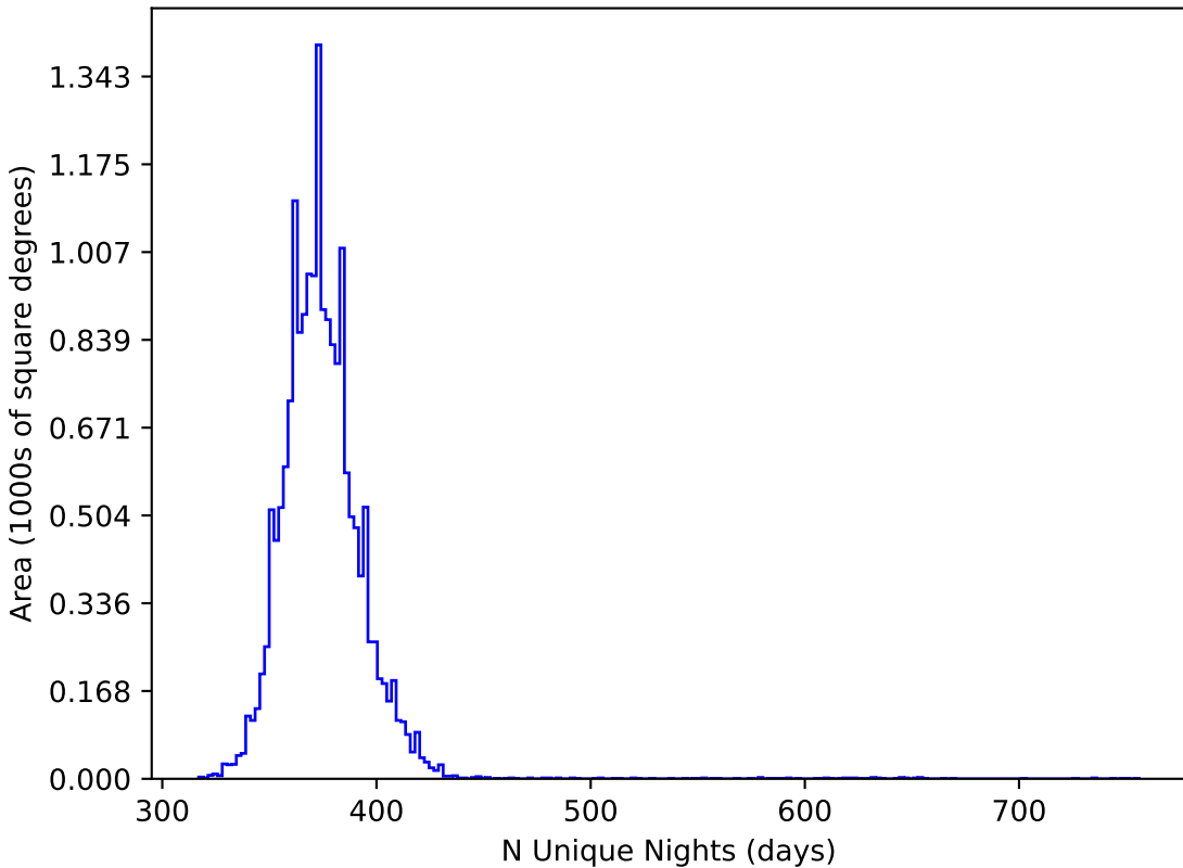
too_5_4v3.4_10yrs WFD all bands: N Unique Nights
