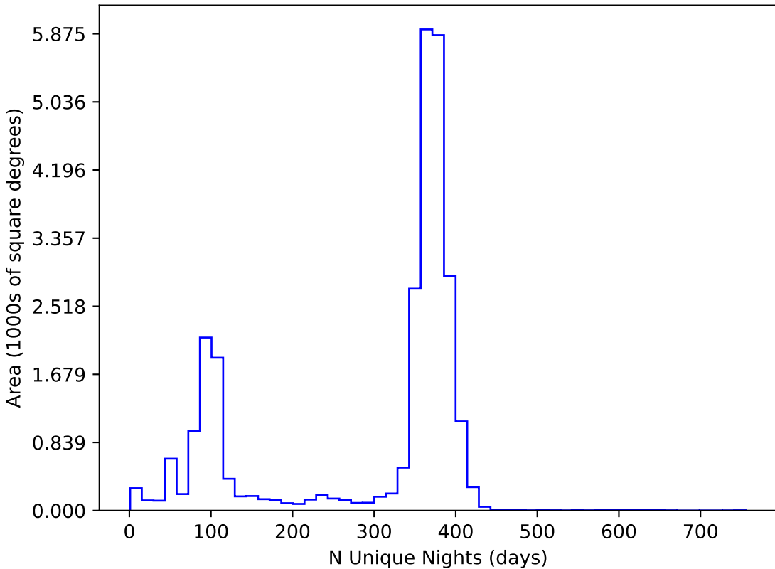
too_5_4v3.4_10yrs All sky all bands: N Unique Nights
