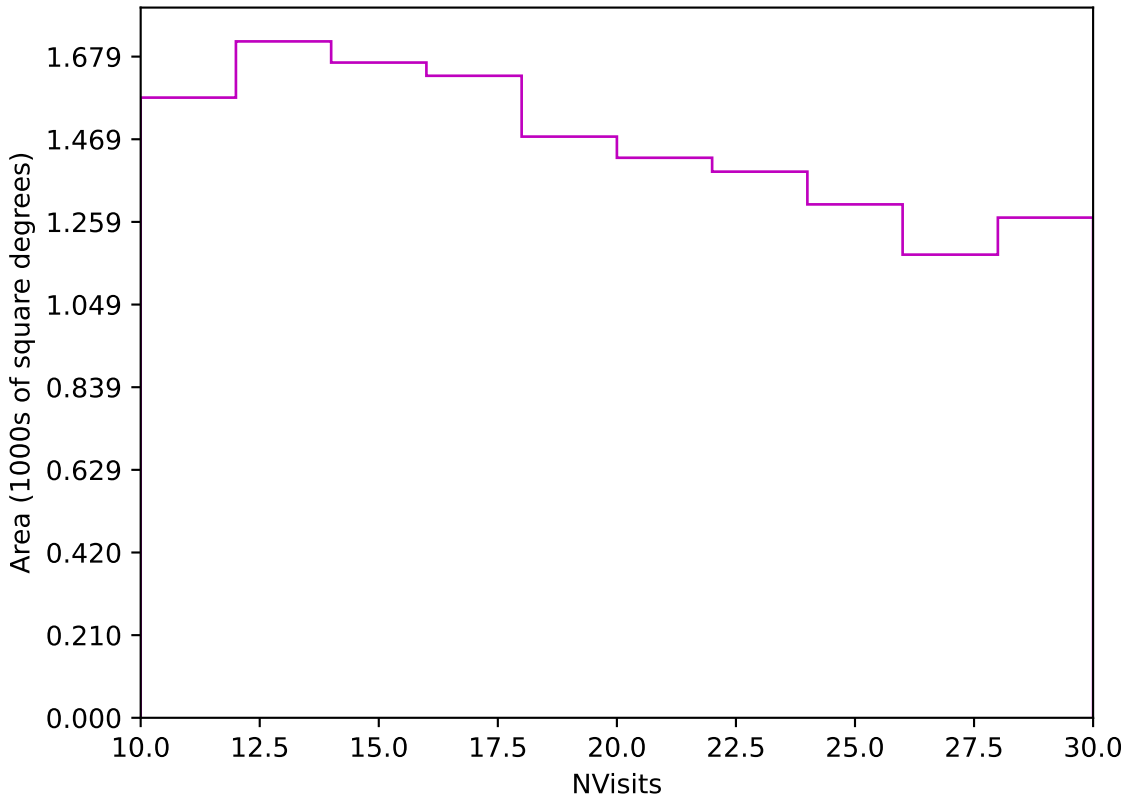
too_5_4v3.4_10yrs Yr 3-4 z band: NVisits
