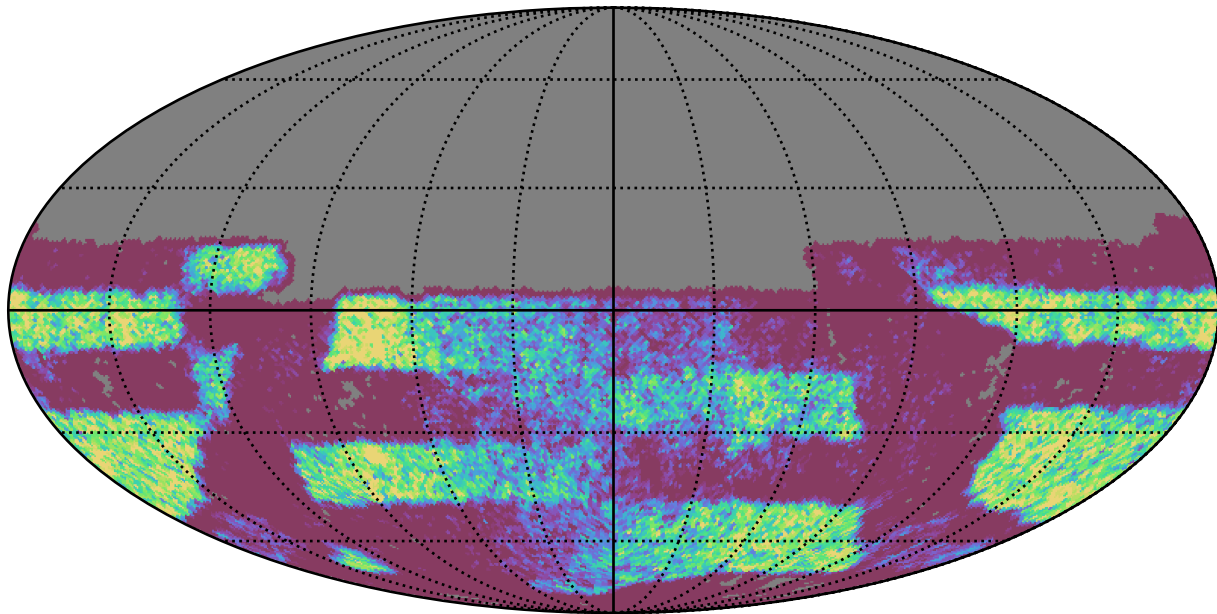
too_5_4v3.4_10yrs Yr 3-4 y band: NVisits
