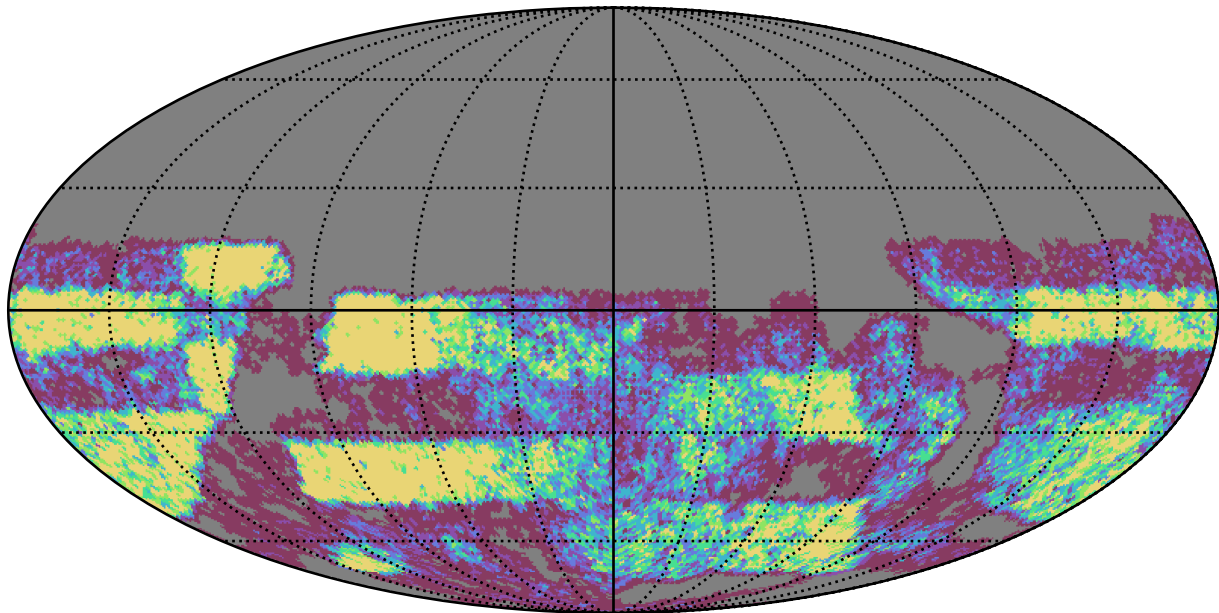
too_5_4v3.4_10yrs Yr 3-4 u band: NVisits
