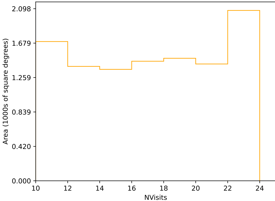
too_5_4v3.4_10yrs Yr 3-4 r band: NVisits
