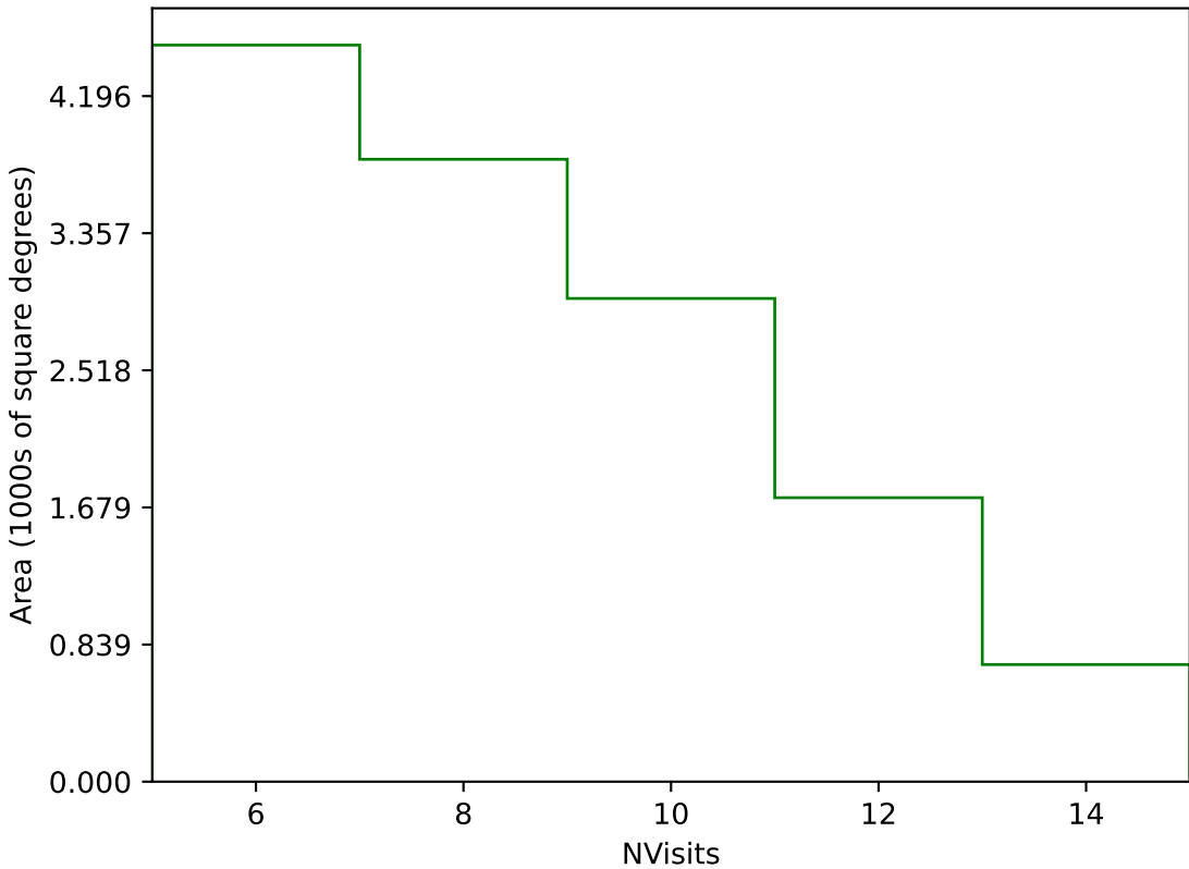
too_5_4v3.4_10yrs Yr 3-4 g band: NVisits
