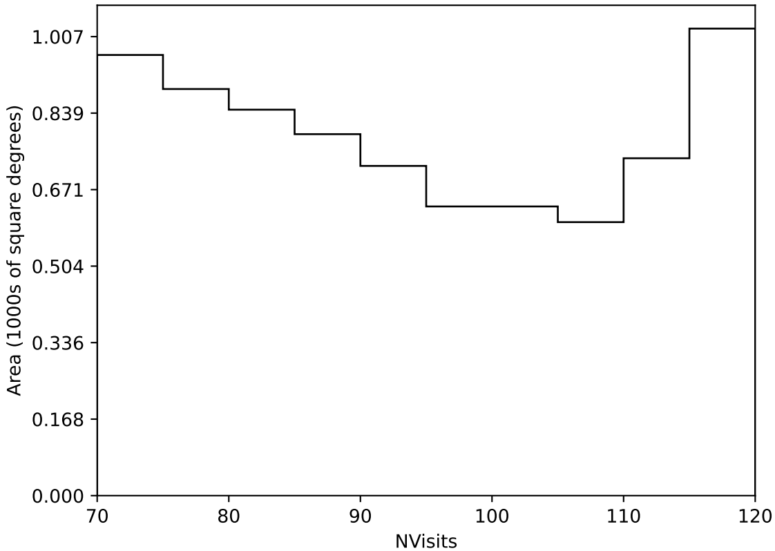
too_5_4v3.4_10yrs Yr 3-4 all bands: NVisits
