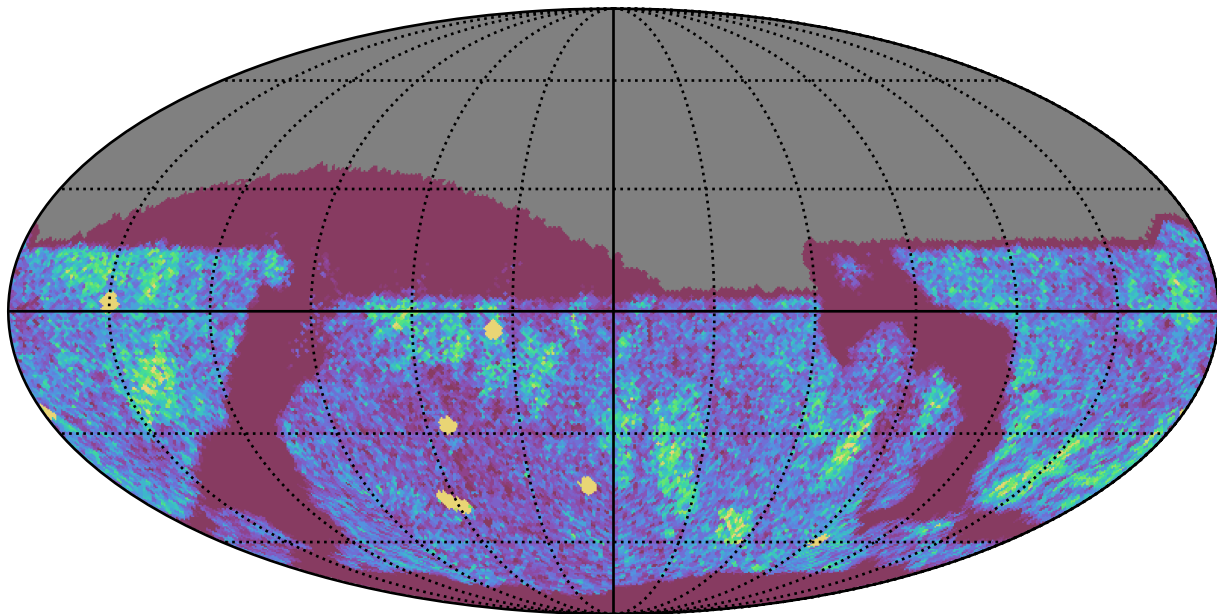
too_5_4v3.4_10yrs Yr 1 z band: NVisits
