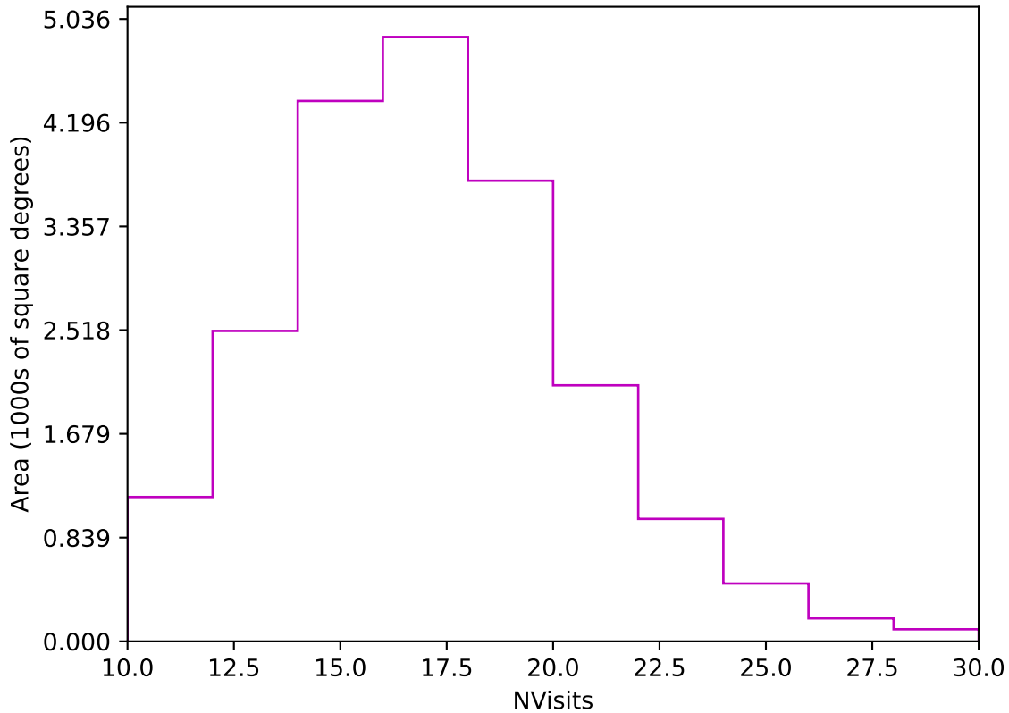
too_5_4v3.4_10yrs Yr 1 z band: NVisits
