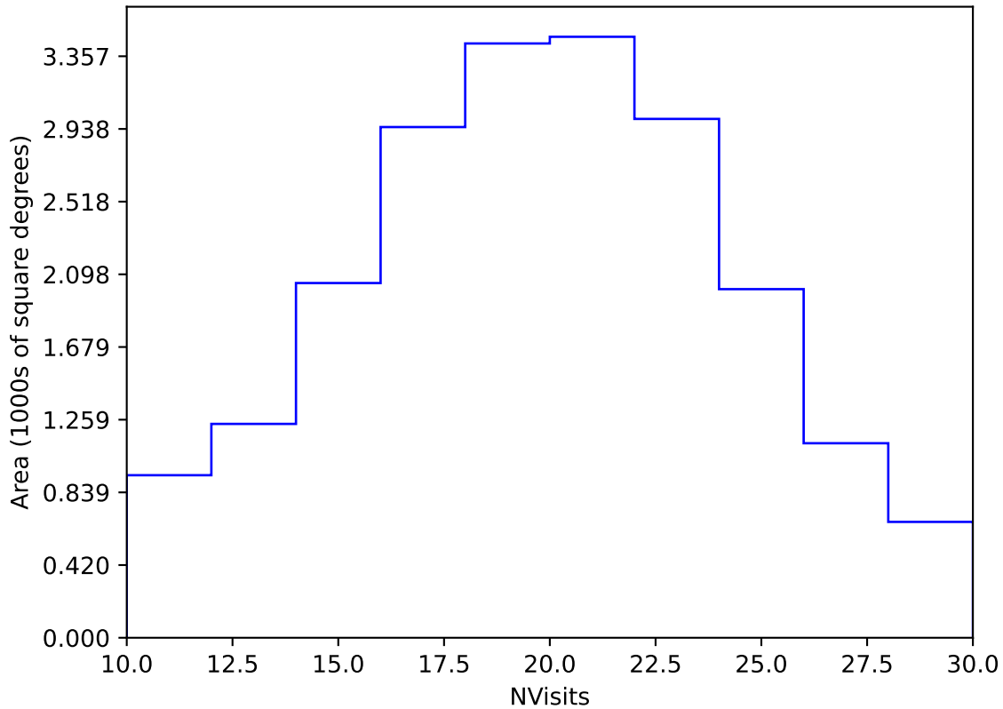
too_5_4v3.4_10yrs Yr 1 y band: NVisits
