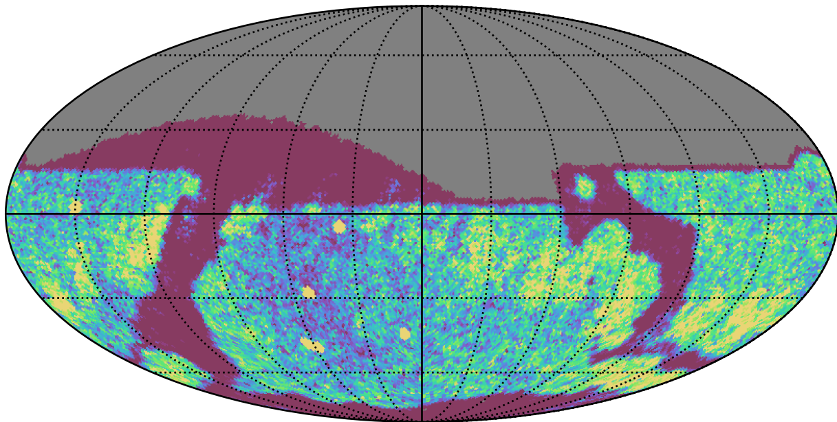
too_5_4v3.4_10yrs Yr 1 r band: NVisits
