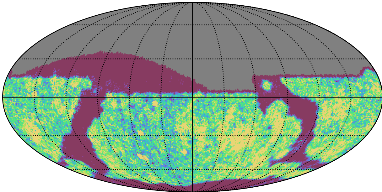
too_5_4v3.4_10yrs Yr 1 i band: NVisits
