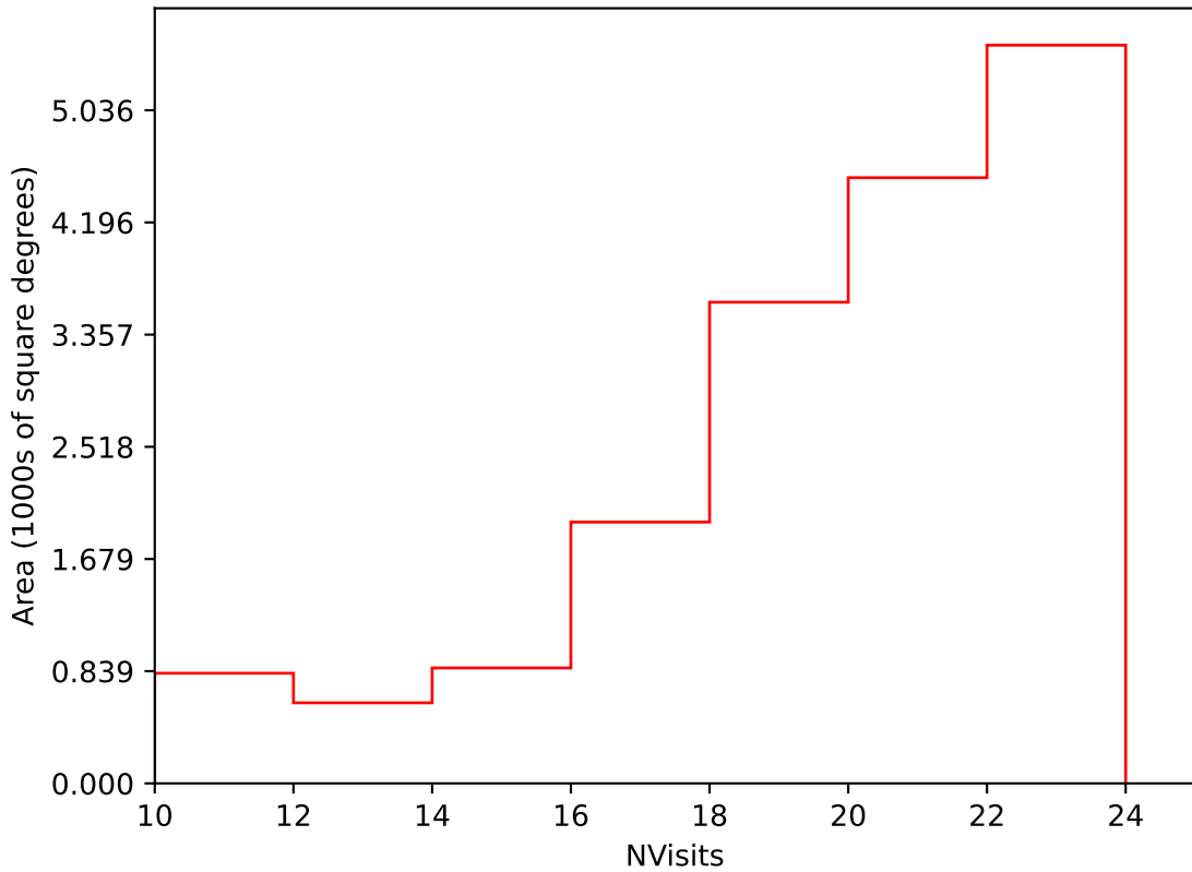
too_5_4v3.4_10yrs Yr 1 i band: NVisits
