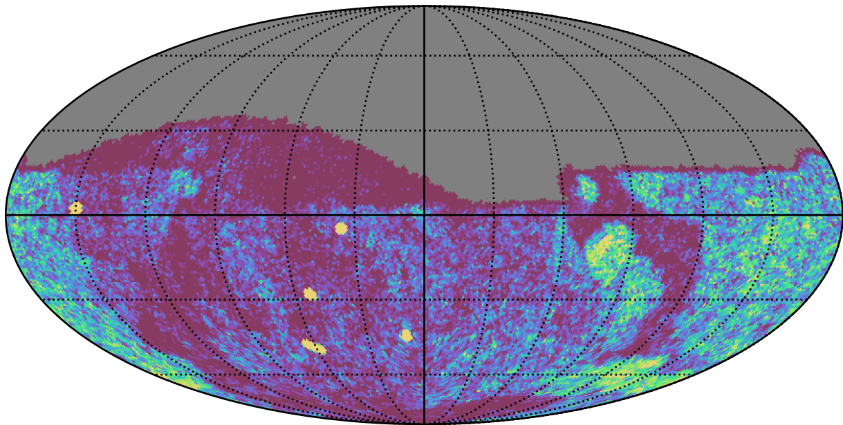
too_5_4v3.4_10yrs Yr 1 g band: NVisits
