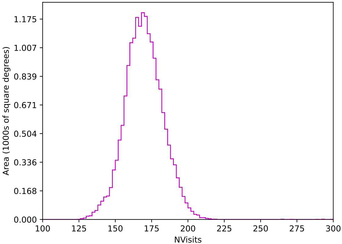
too_5_4v3.4_10yrs WFD z band: NVisits
