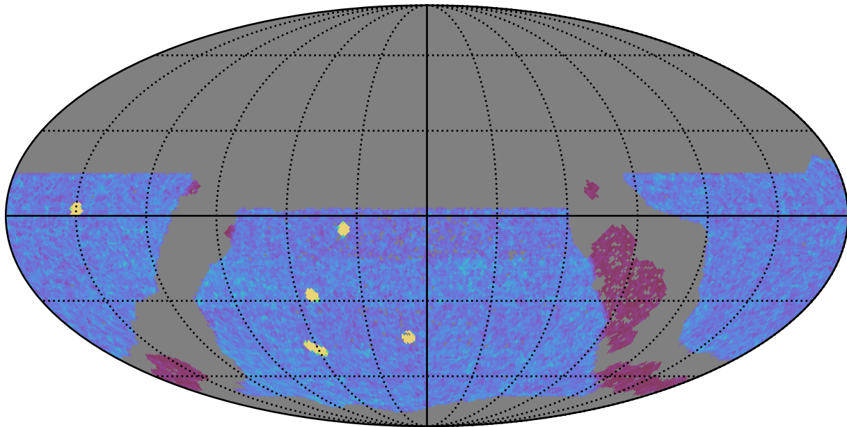
too_5_4v3.4_10yrs WFD y band: NVisits
