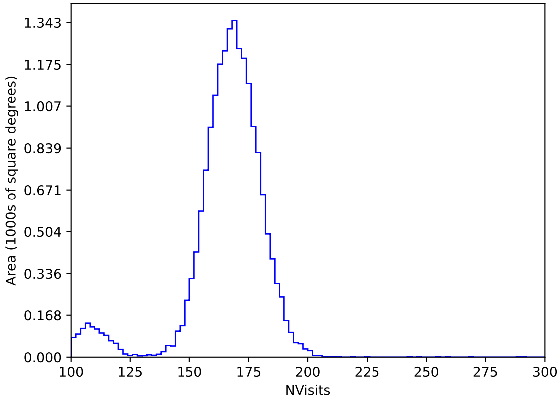
too_5_4v3.4_10yrs WFD y band: NVisits
