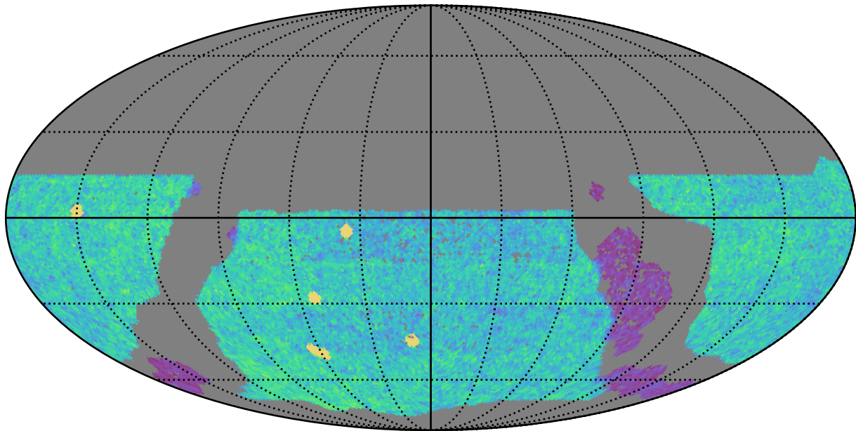
too_5_4v3.4_10yrs WFD u band: NVisits
