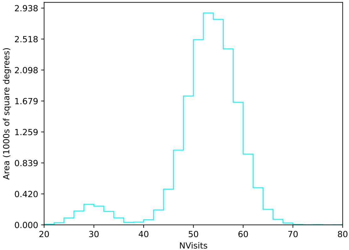
too_5_4v3.4_10yrs WFD u band: NVisits
