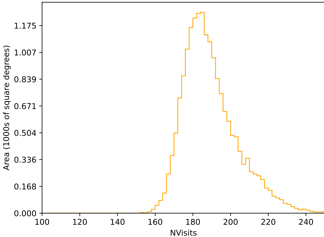
too_5_4v3.4_10yrs WFD r band: NVisits
