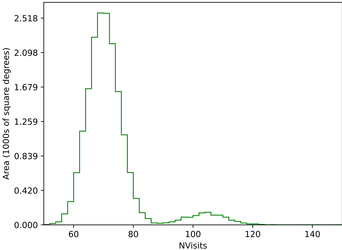
too_5_4v3.4_10yrs WFD g band: NVisits
