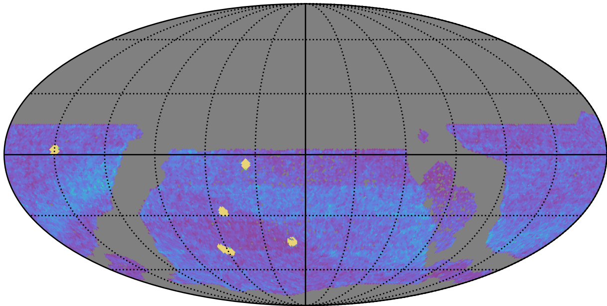
too_5_4v3.4_10yrs WFD all bands: NVisits
