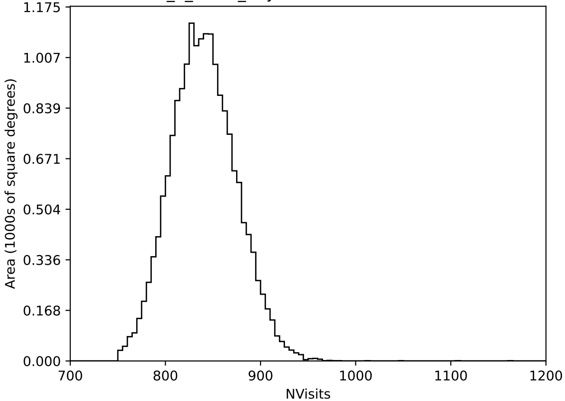
too_5_4v3.4_10yrs WFD all bands: NVisits
