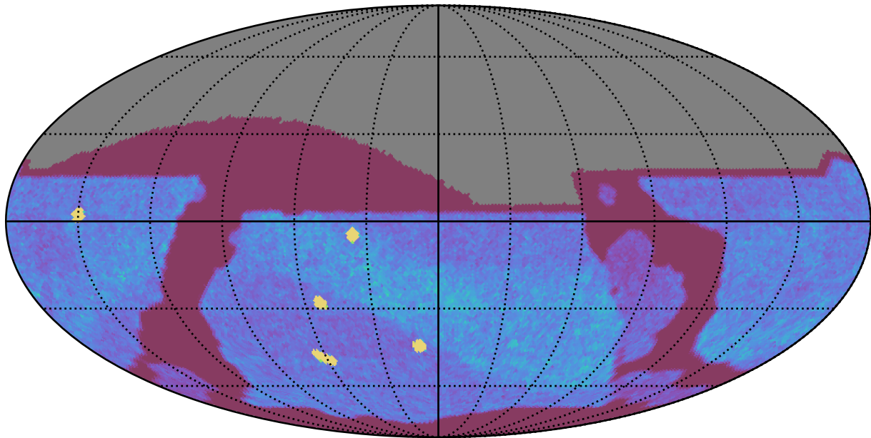
too_5_4v3.4_10yrs All sky z band: NVisits
