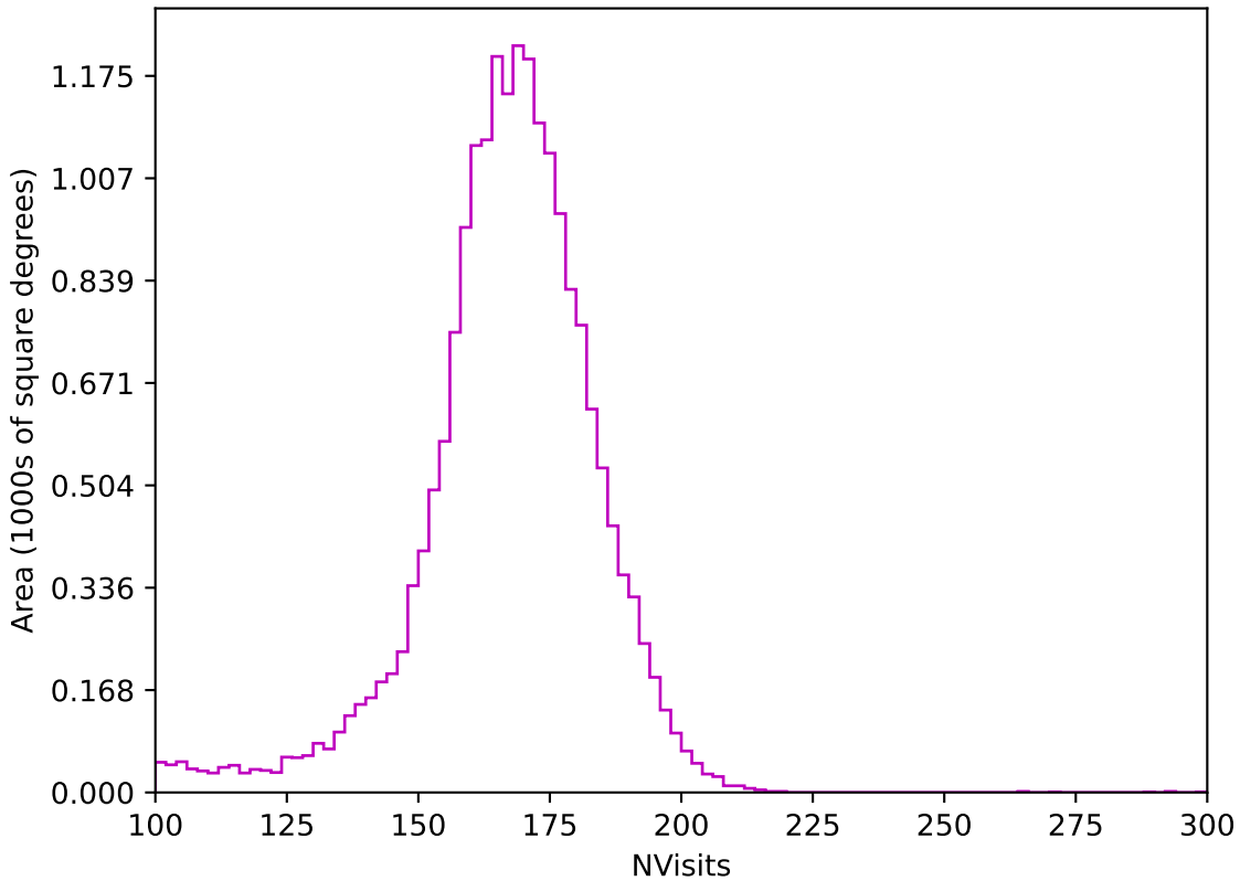
too_5_4v3.4_10yrs All sky z band: NVisits
