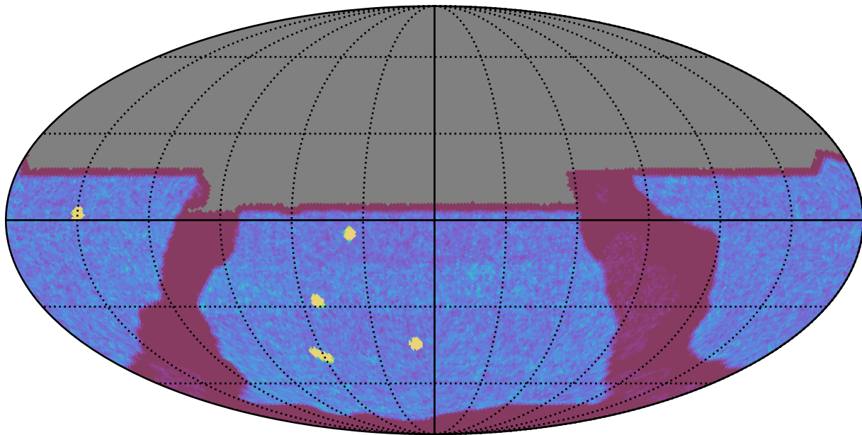
too_5_4v3.4_10yrs All sky y band: NVisits
