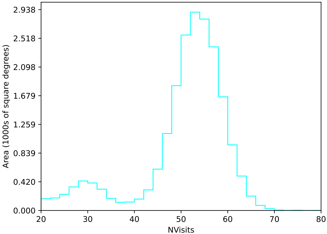
too_5_4v3.4_10yrs All sky u band: NVisits
