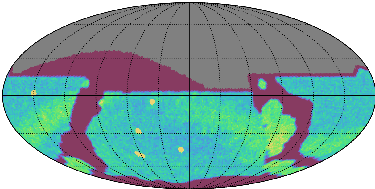
too_5_4v3.4_10yrs All sky r band: NVisits
