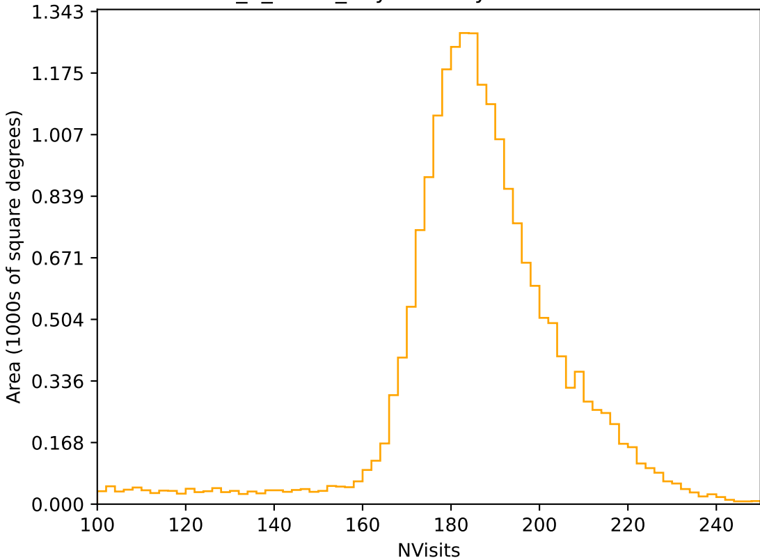
too_5_4v3.4_10yrs All sky r band: NVisits
