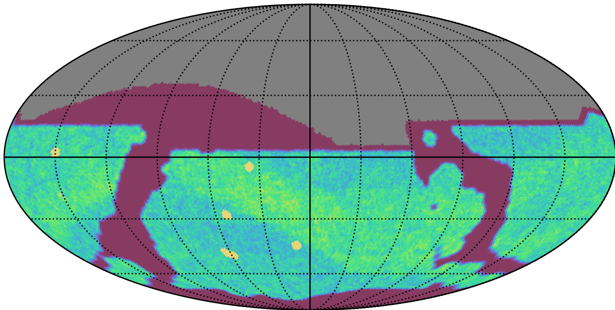
too_5_4v3.4_10yrs All sky i band: NVisits
