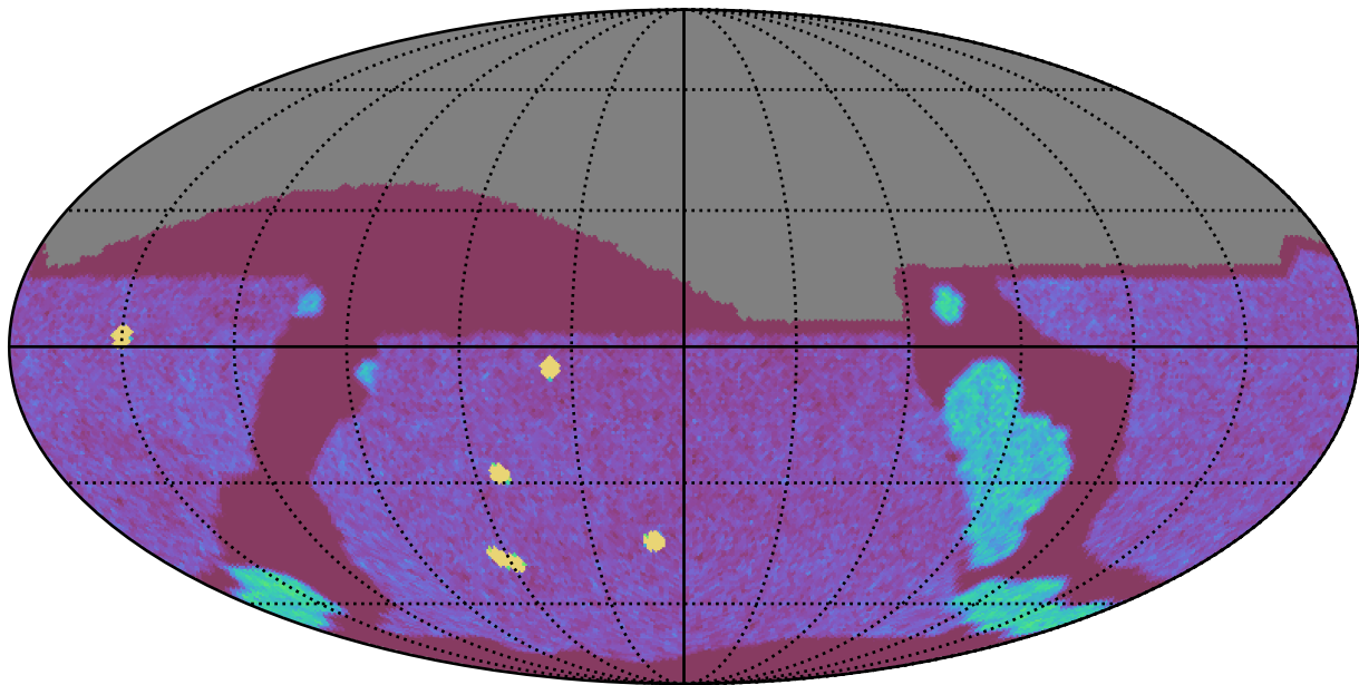
too_5_4v3.4_10yrs All sky g band: NVisits
