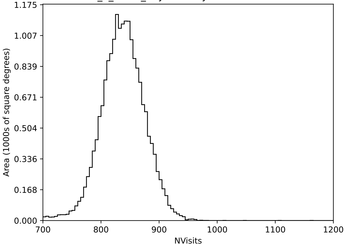
too_5_4v3.4_10yrs All sky all bands: NVisits
