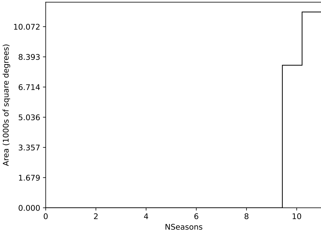
too_5_4v3.4_10yrs WFD all bands: NSeasons
