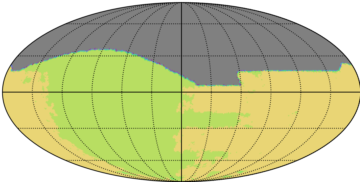
too_5_4v3.4_10yrs All sky all bands: NSeasons
