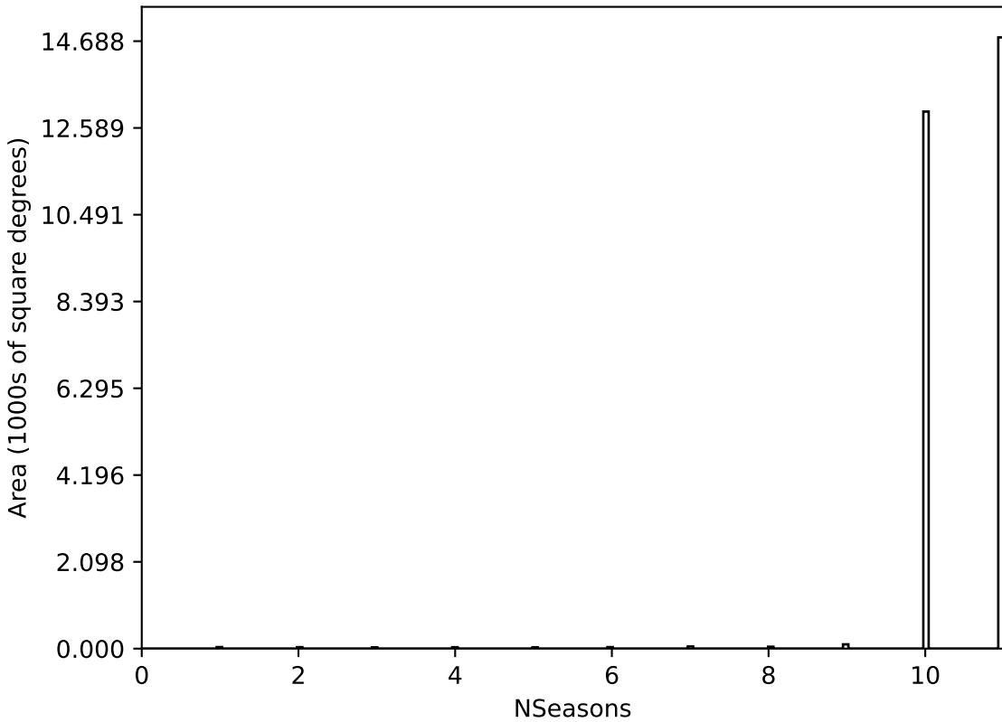
too_5_4v3.4_10yrs All sky all bands: NSeasons
