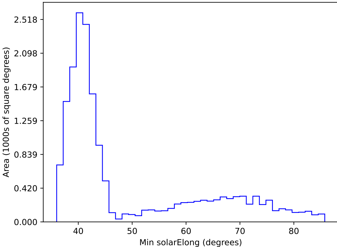
too_5_4v3.4_10yrs WFD z band: Min solarElong
