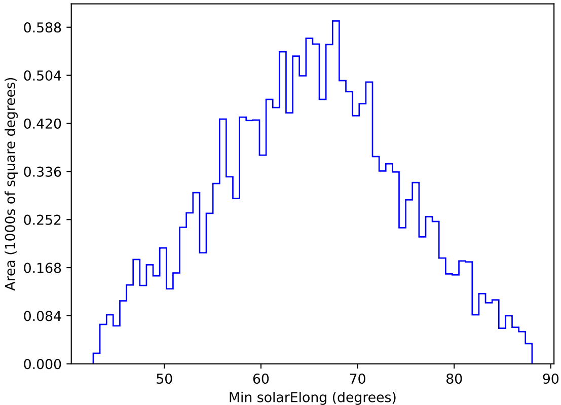
too_5_4v3.4_10yrs WFD y band: Min solarElong
