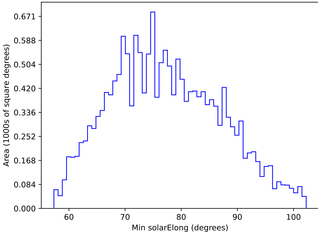
too_5_4v3.4_10yrs WFD u band: Min solarElong
