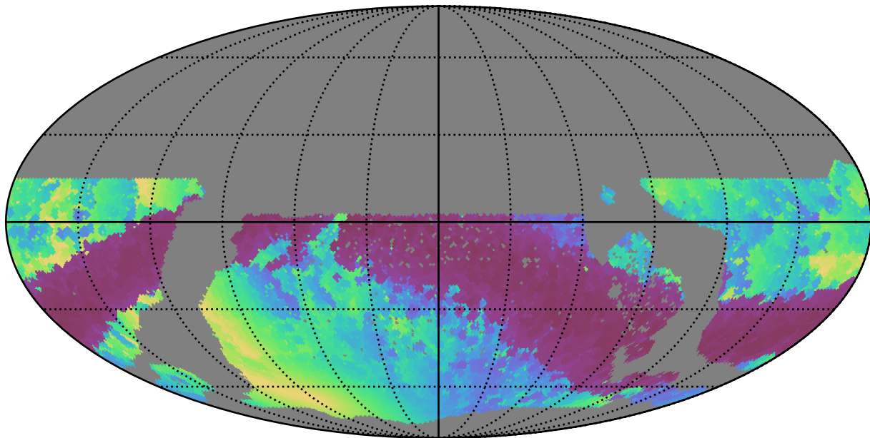
too_5_4v3.4_10yrs WFD r band: Min solarElong
