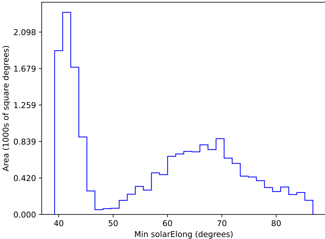
too_5_4v3.4_10yrs WFD r band: Min solarElong
