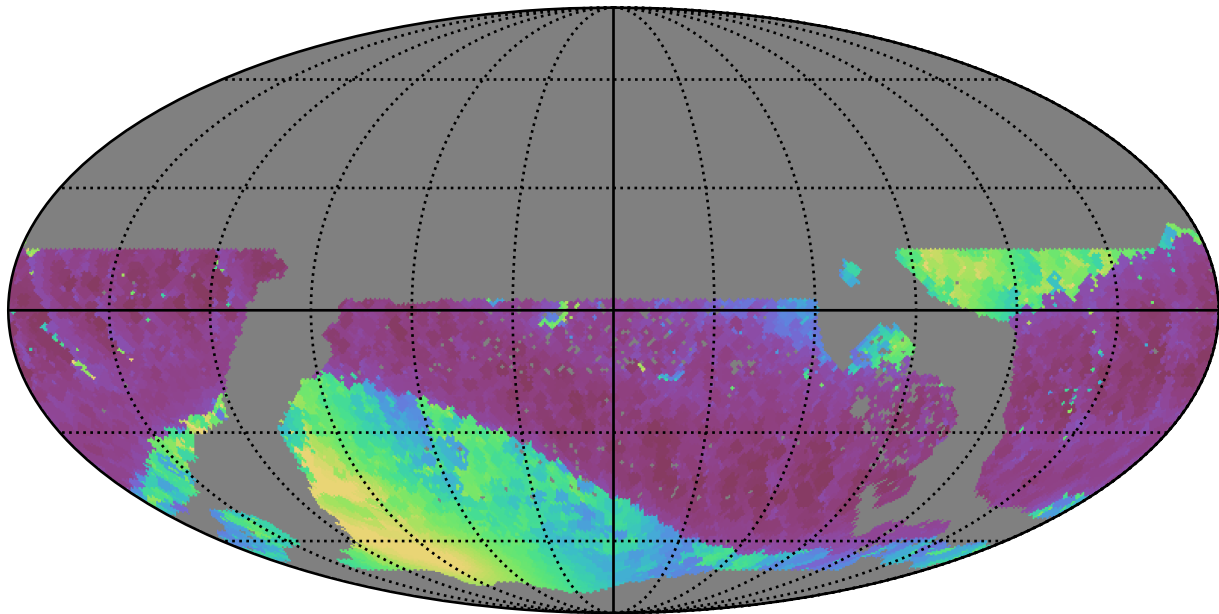
too_5_4v3.4_10yrs WFD i band: Min solarElong
