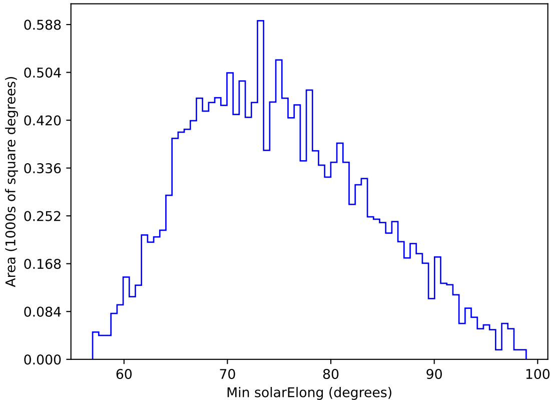
too_5_4v3.4_10yrs WFD g band: Min solarElong
