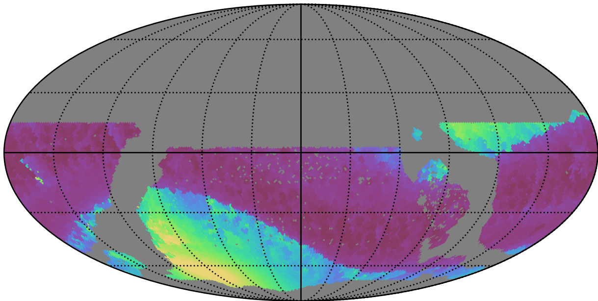
too_5_4v3.4_10yrs WFD all bands: Min solarElong
