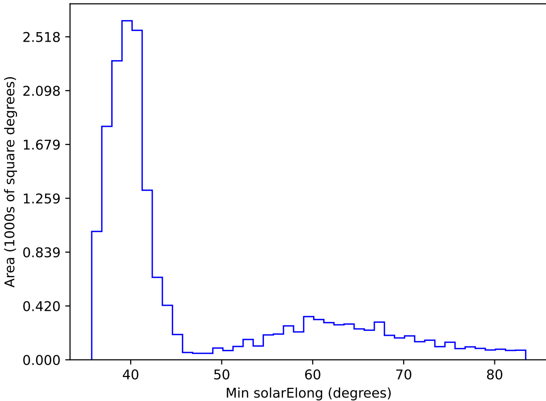
too_5_4v3.4_10yrs WFD all bands: Min solarElong
