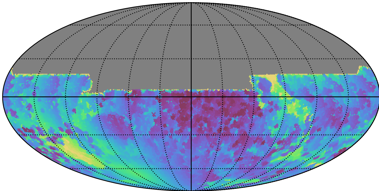
too_5_4v3.4_10yrs All sky y band: Min solarElong
